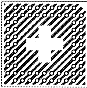
FIGURE 9 — HOLE SIDE OF A MARKED 68-PIN SOCKET
